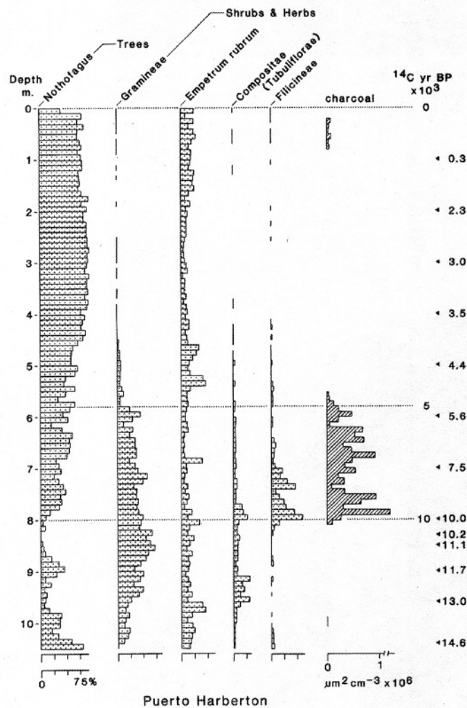
FIGURE 15 – Diagram of principal pollen-spore taxa shown in relation to charcoal in the mire section at Puerto Harberton, Argentina (redrawn from HEUSSER, 1994).
