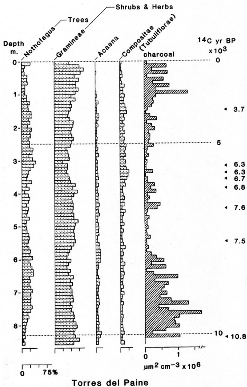
FIGURE 19 – Diagram of principal pollen taxa and charcoal in the section of limnic sediments from the summer-dry lake at Torres del Paine, Chile (redrawn from HEUSSER, 1994)..
