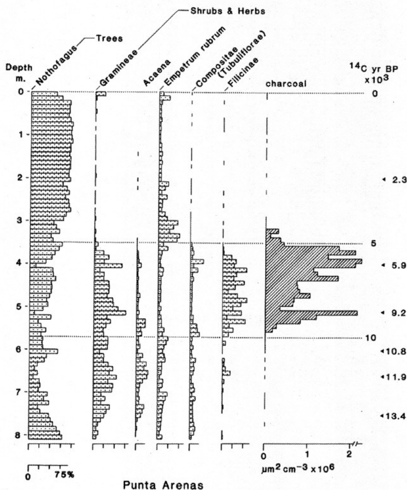
FIGURE 18 – Diagram of principal pollen-spore taxa and charcoal in the mire section at Punta Arenas, Chile (redrawn from HEUSSER, 1994).
