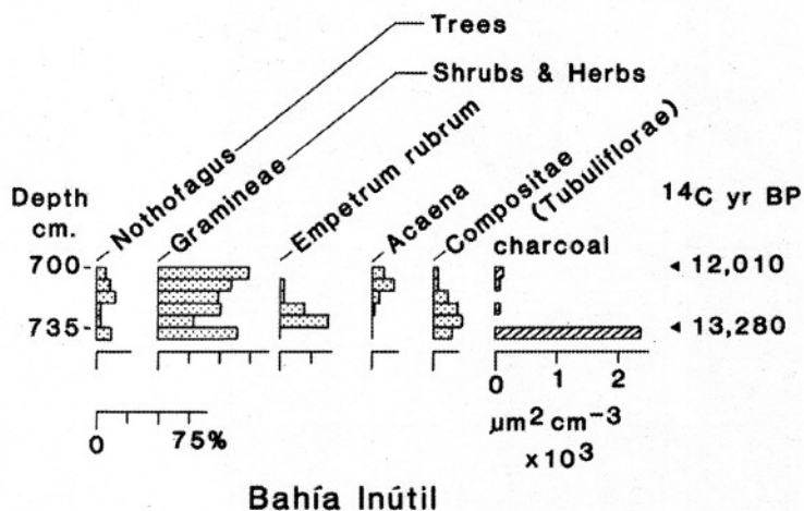
FIGURE 17 – Diagram of major pollen taxa and charcoal in the lacustrine sequence at Bahía Inútil, Chile (redrawn from HEUSSER, 1994).
