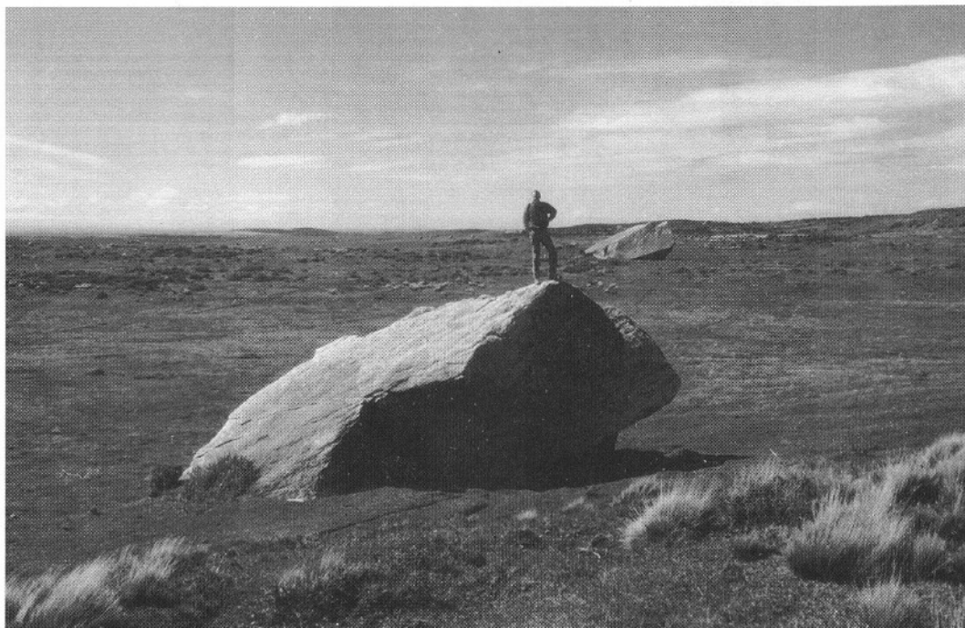
FIGURE 12 – Granite erratics, glacially transported from the core of the Andes in the Cordillera Darwin, weathering out of drift along the southern border of Bahía Inútil, Isla Grande.
