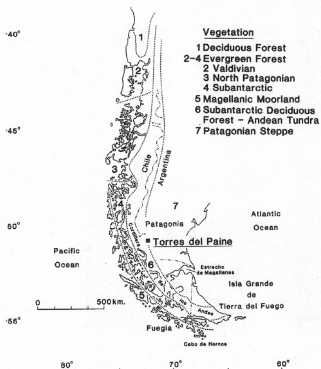
FIGURE 1 – Location of Fuegia and Patagonia, including site of Torres del Paine, in relation to vegetation zones (SCHMITHÜSEN, 1960; PISANO, 1977, 1981; MOORE, 1983).
