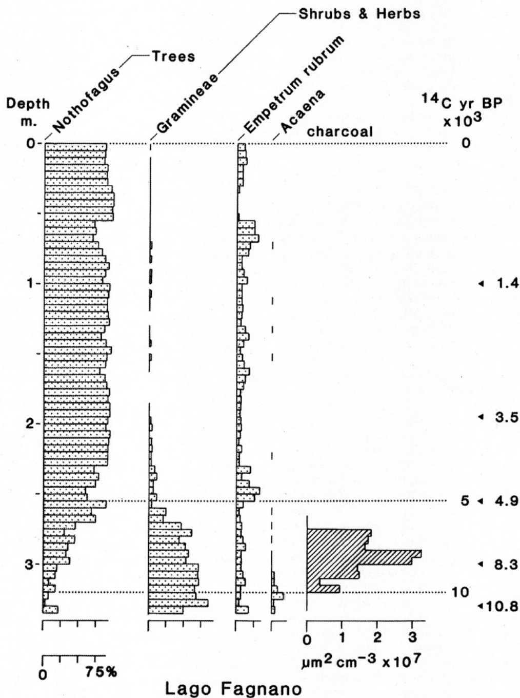
FIGURE 16 – Diagram of principal pollen taxa and charcoal in the section of mire at Lago Fagnano, Argentina (redrawn from HEUSSER, 1994).
