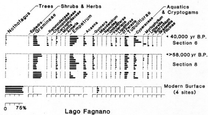
FIGURE 14 – Pollen-spore diagram of biogenic lacustrine sediments exposed in topset beds of the proglacial delta at Lago Fagnano. Fossil spectra in sections 6 and 8 are compared with modern spectra at four nearby sites located in Subantarctic Deciduous Forest. Noteworthy taxa are indicated by enlarged type.
