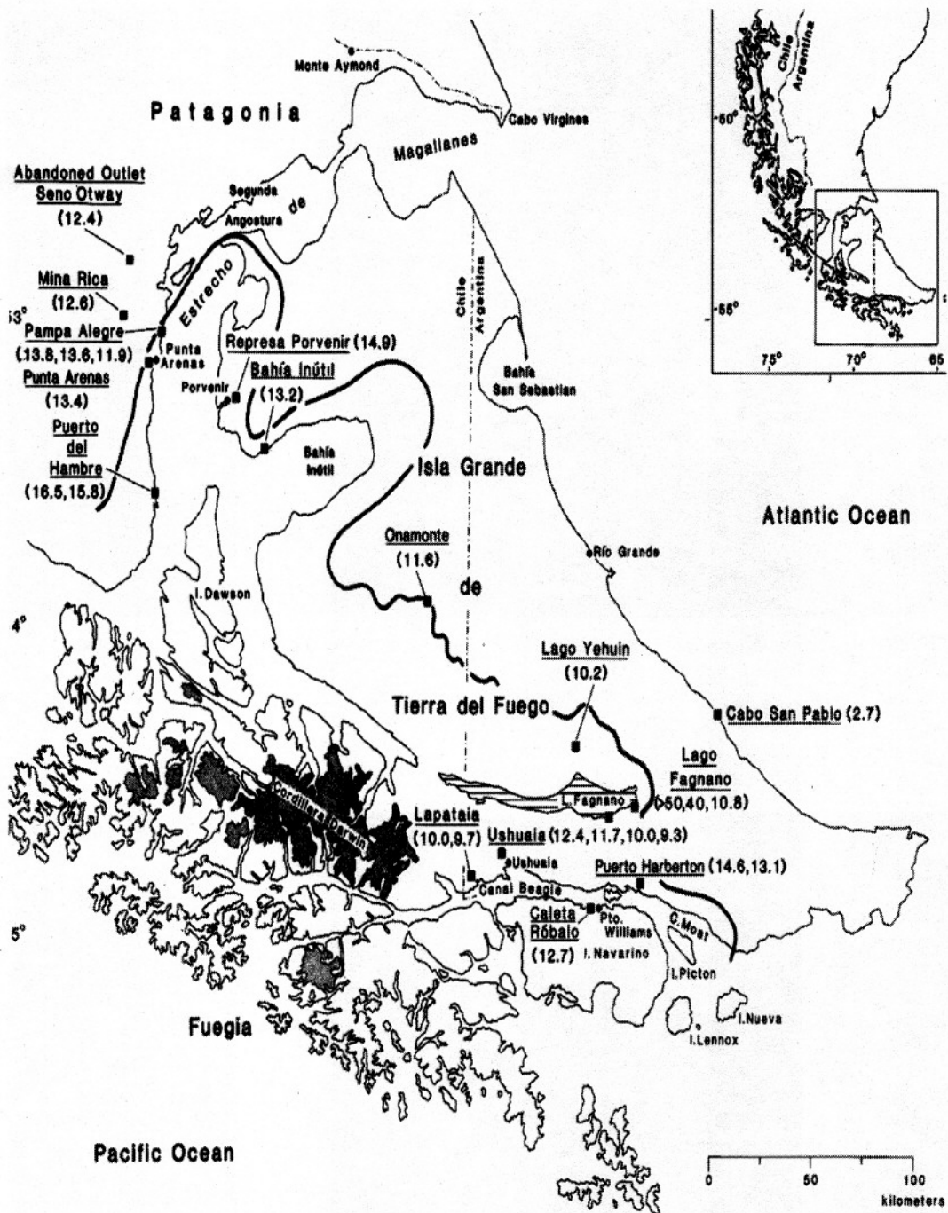
FIGURE 9 – Extent of glaciation on Isla Grande de Tierra del Fuego during the last glacial maximum, shown approximately by heavy solid line. Lobes advanced in the Estrecho de Magallanes, Bahía Inútil, Lago Fagnano, and Canal Beagle. Existing areas of glaciers, notably in the Cordillera Darwin, are indicated by stippling. Study sites with radiocarbon dates ( \times 10^3 yr BP) appear underlined. See text for sources.
